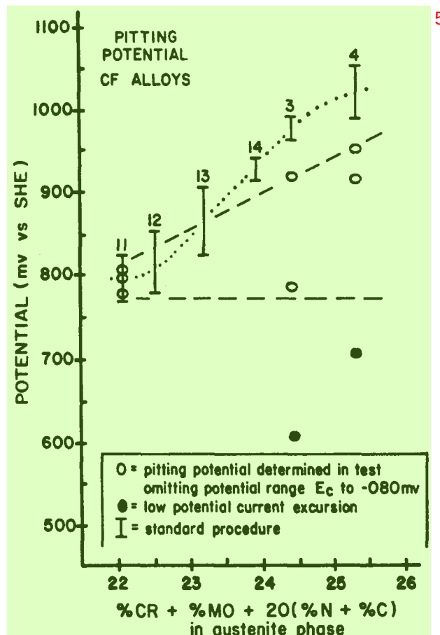
FIGURE 12. Comparison of pitting potentials determined from the standard cyclic polarization test with pitting potentials determined from testing which limits the influence of the low potential loop in the scan procedure.
