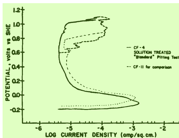
FIGURE 5. CPPT curve for solution-treated CF-4 (high-nitrogen alloy).
